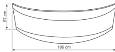
Front panel - Prednja obloga
